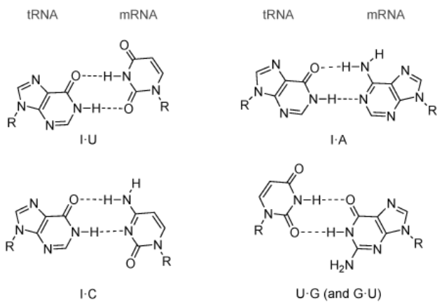
Figure 12 | Structures of wobble base pairs found in RNA
