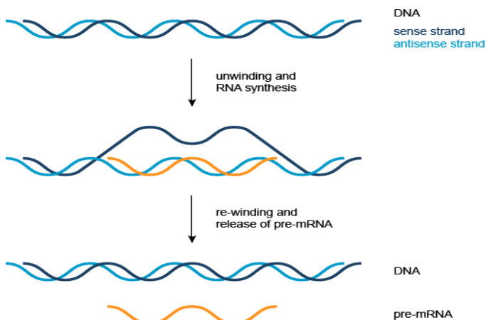
Figure 4 | Transcription Simplified representation of the formation of pre-messenger RNA (orange) from double-stranded DNA (blue) in transcription.
